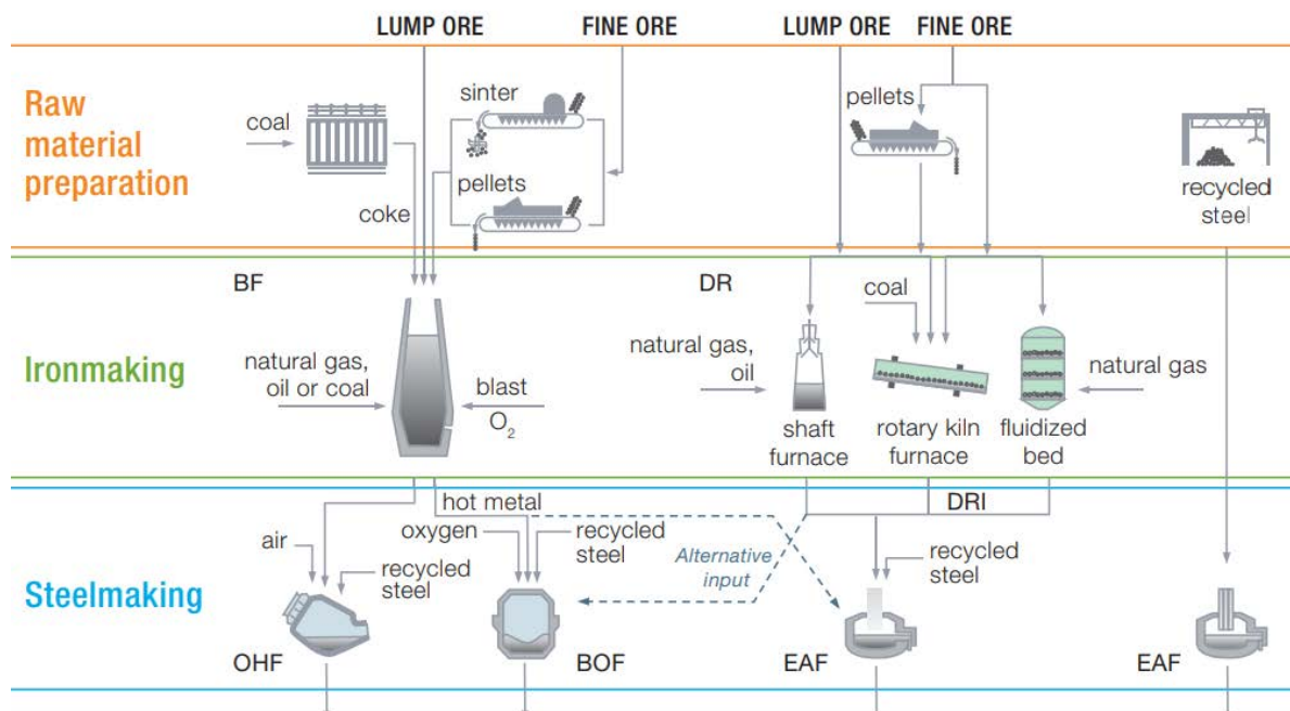
Figure 25 Steelmaking routes 121
